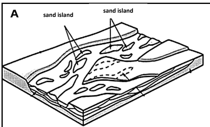
FIGURE 2.6: FLUVIAL LANDFORMS
