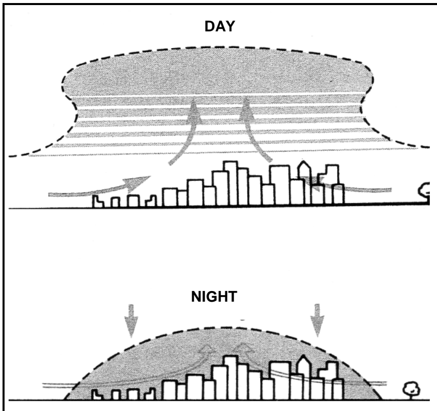
FIGURE 2.3: HEAT ISLAND
