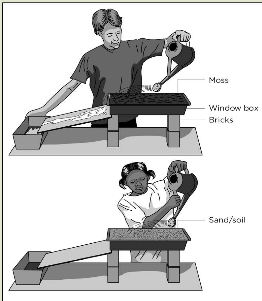
Setup for the drainage experiment.
